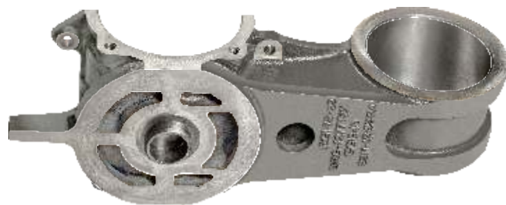
RG-R201 Control Arm Upper SG 400/18 specially for LHB coaches Indian Railway
